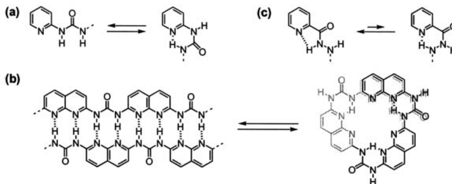
Figure 13. a) cis-trans equilibrium of 2-ureopyridines; b) equilibrium between intramolecularly hydrogen-bonded linear and helical monomers; c) for comparison the cis-trans equilibrium for 2-pyridinecarboxylic acid hydrazide
