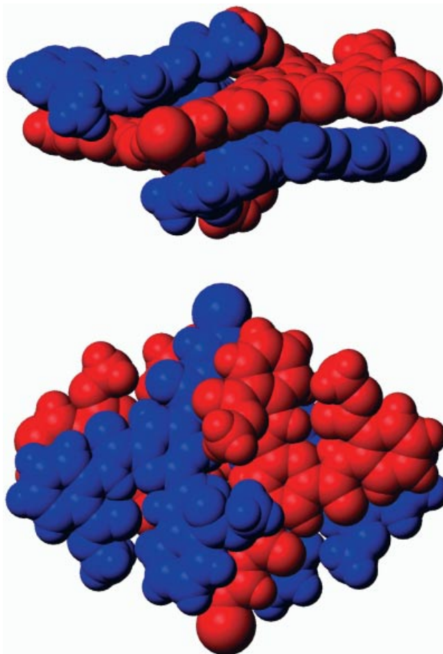
Figure 16. Side and top views of the intertwined dimer of the second-generation dendrimer represented in Figure 5 (a)
