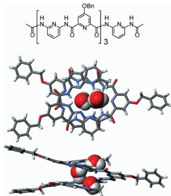
Figure 10. Crystal structure of an oligomer showing water molecules included in a polar helix groove
