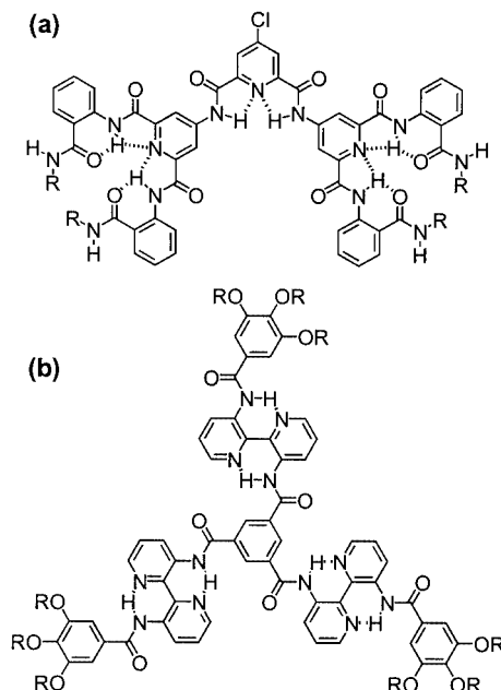
Figure 5. Examples of branched aromatic oligoamide foldamers; a crystal structure of the dendrimer shown in (a) is represented in Figure 16
