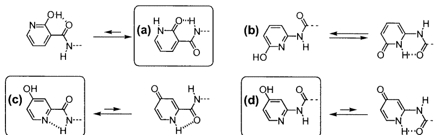
Figure 14. Lactam-lactim tautomerization
