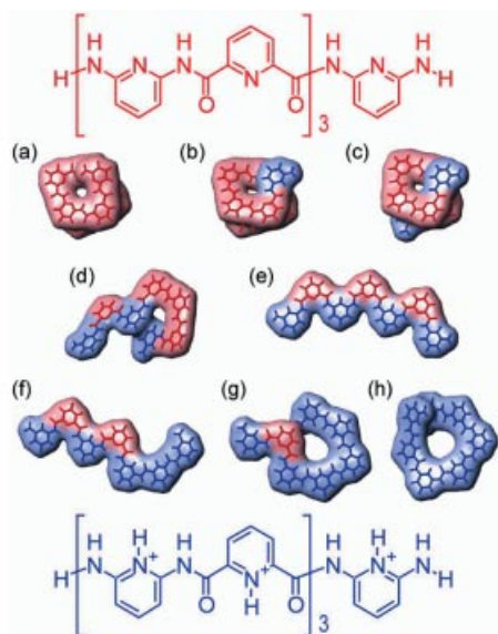
Figure 12. Energy-minimized structures of the various protonated states of an oligoamide comprising four 2,6-diaminopyridine units alternating with three 2,6-pyridinedicarboxyl units; the protonated rings are shown in blue while rings which are not protonated are in red
