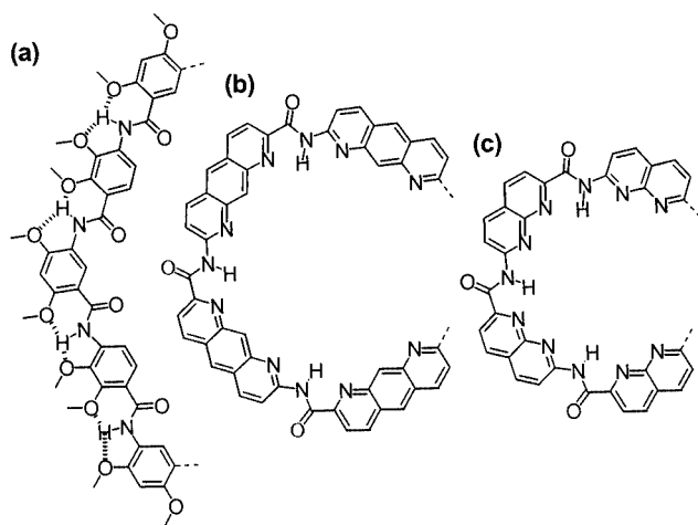
Figure 9. Tuning strand bending
