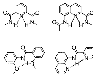
Figure 3. Examples of hydrogen bonds involving two protons and one acceptor (top) or one proton and two acceptors (bottom)
