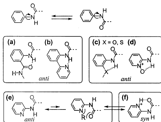
Figure 2. Conformational preferences of various CONH–aryl linkages; “R” denotes electrostatic repulsions
