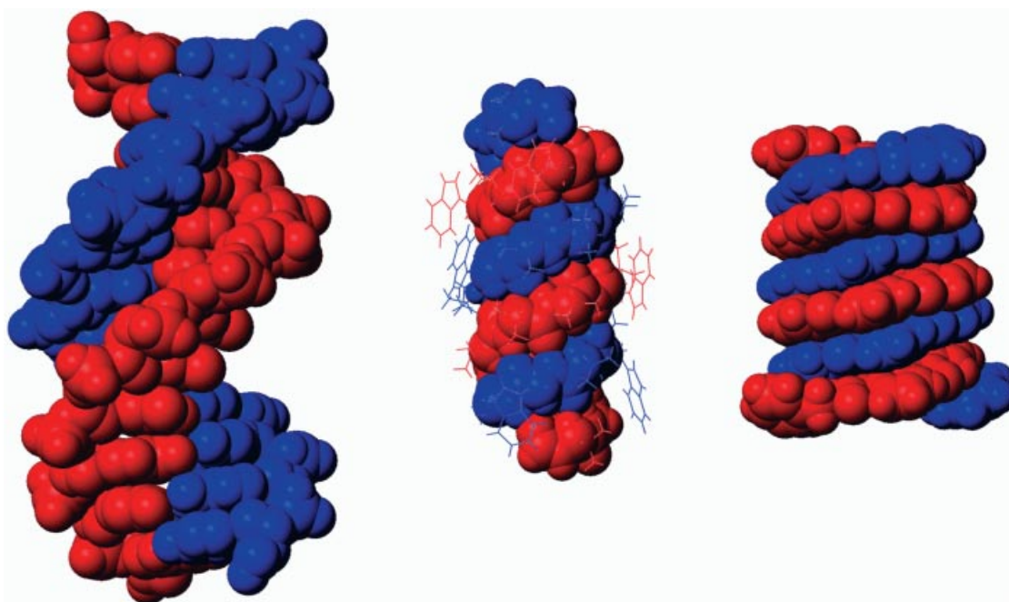
Figure 17. Side (top) and top (center) views of three crystal structures of two oligoamides of 2,6-diaminopyridine and 2,6-pyridinedicarboxylic acid (bottom); the three structures are represented on the same scale; non-amide hydrogen atoms and included solvent molecules have been omitted for clarity
