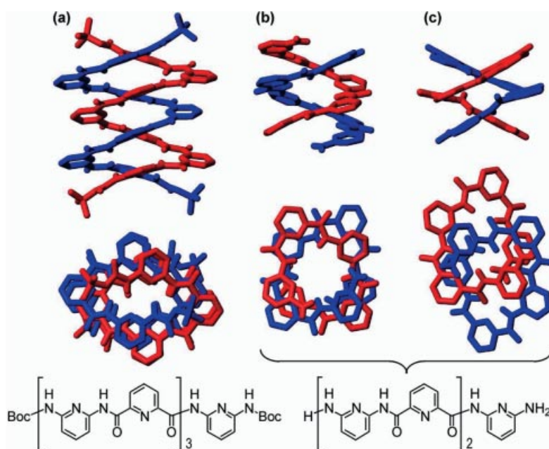
Figure 17. Side (top) and top (center) views of three crystal structures of two oligoamides of 2,6-diaminopyridine and 2,6-pyridinedicarboxylic acid (bottom); the three structures are represented on the same scale; non-amide hydrogen atoms and included solvent molecules have been omitted for clarity
