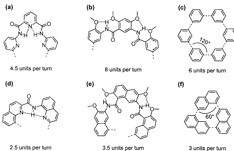
Figure 8. Bending of aromatic oligomers depends on intramolecular hydrogen bonds on the inner or outer rim of the oligomer, and on the substitution motif ( ortho , meta , ...) of aromatic rings
