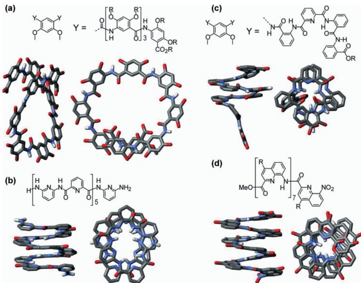
Figure 7. Structures in the solid state of four aromatic oligoamides comprising 8–11 units; the four compounds are represented on the same scale; for clarity, non-amide hydrogen atoms, alkyl groups and included solvent molecules have been omitted; structures (a), (b), (c), and (d) are described in refs.[9,18,28,13]
