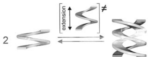
Figure 15. The intertwining equilibrium of helices
