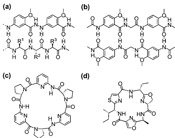
Figure 4. Mixed aliphatic–aromatic oligoamide foldamers
