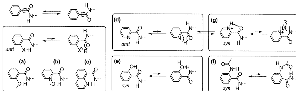
Figure 1. Conformational preferences of various NHCO–aryl linkages; “R” denotes electrostatic repulsions
