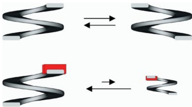
Figure 11. Schematic representation of the equilibria between enantiomeric left- and right-handed helices (top), and between diastereomeric left- and right-handed helices (bottom)
